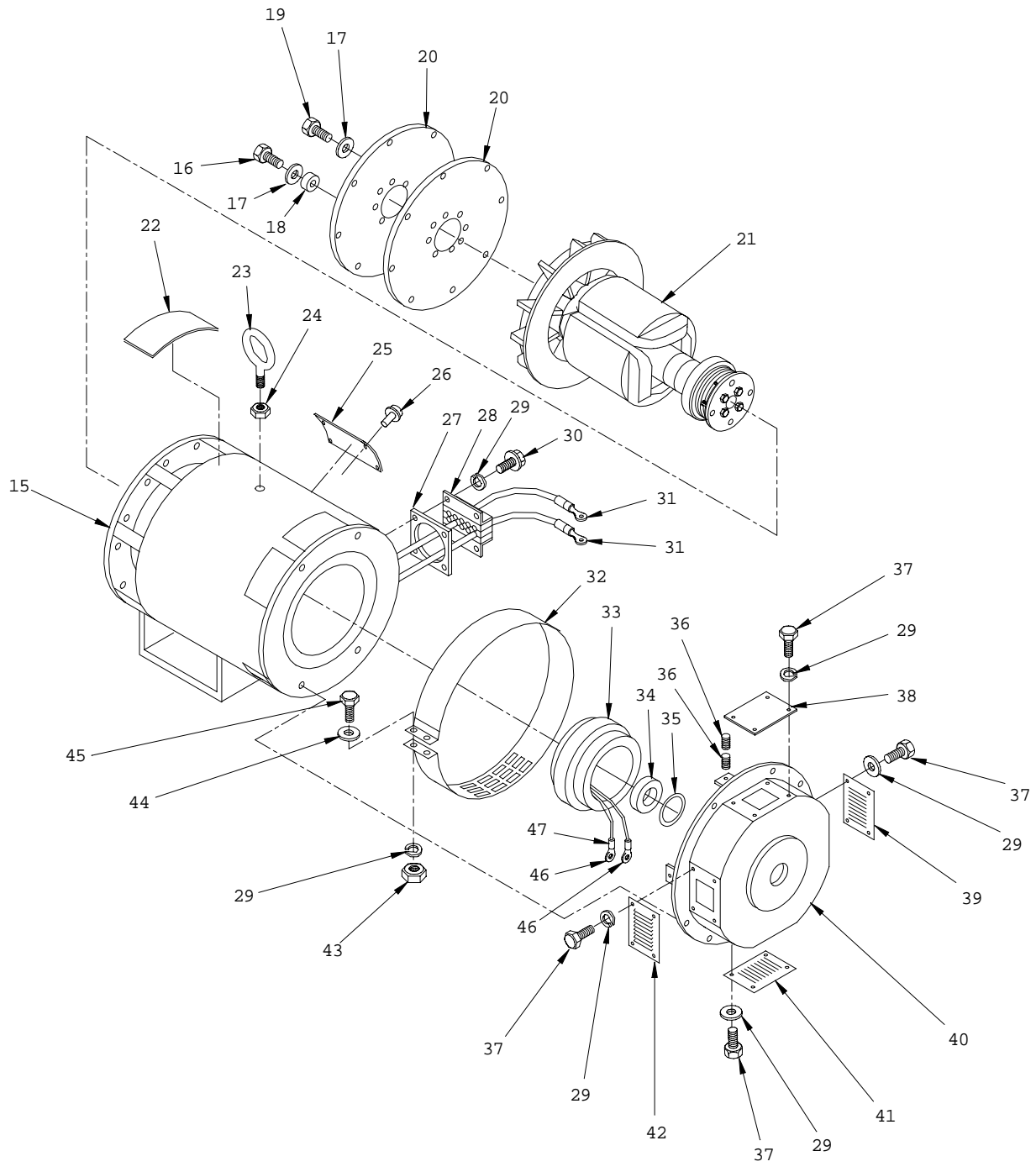
Figure 21. Generator Assembly (Sheet 2 of 2)
