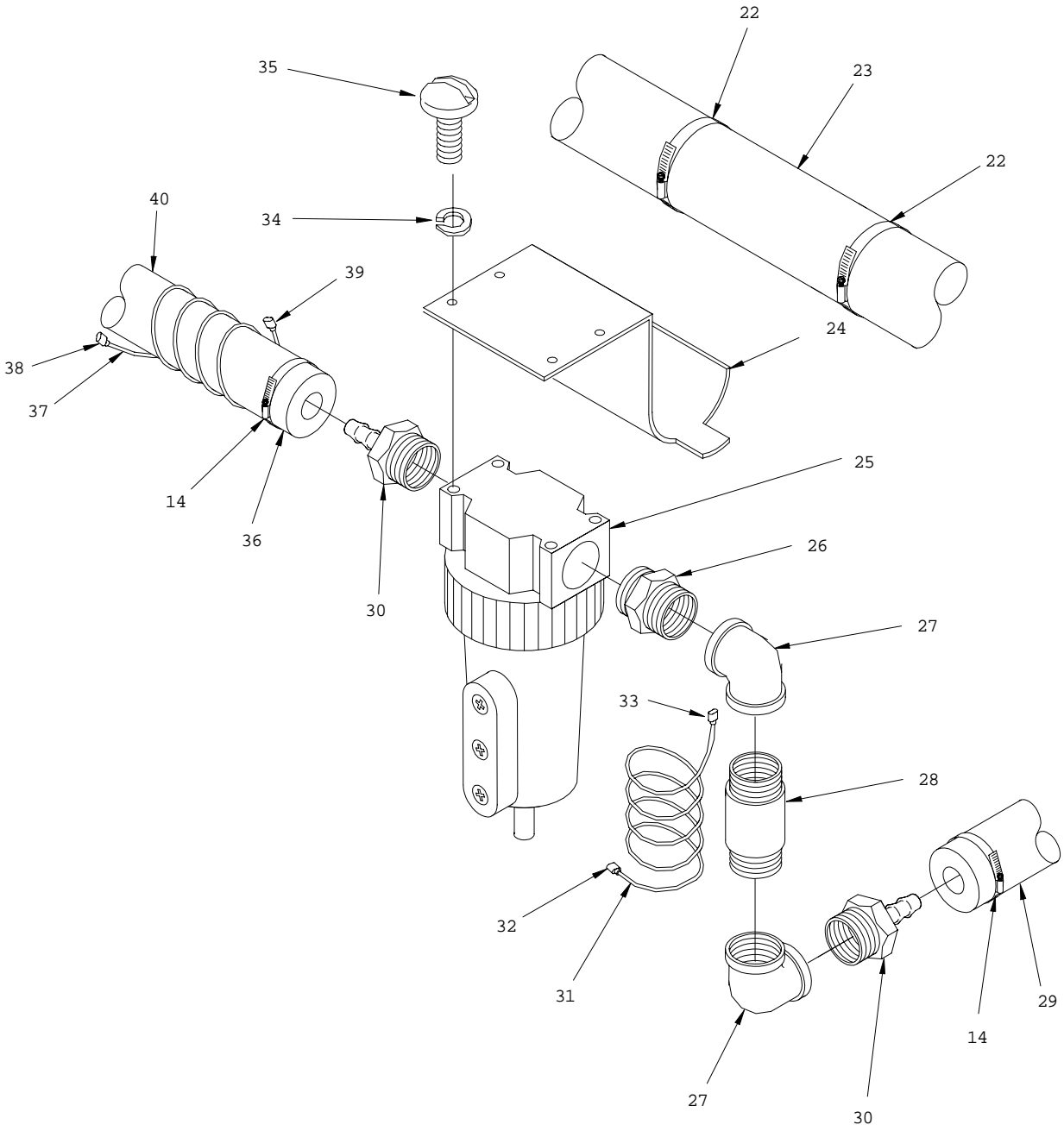
Figure 7. Air Intake and Exhaust System (Sheet 3 of 3)
